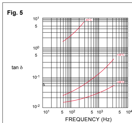
tg δ DRIFT VERSUS FREQUENCY HIGH VOLTAGE (> 100 Vr d.c.)
